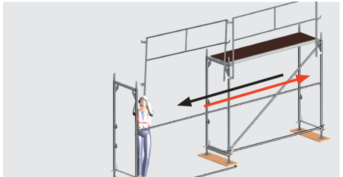
I-Guardrail – system-integrated and can be assembled in both directions
