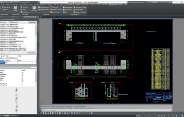
Complex scaffolding planning with LayPLAN CAD
