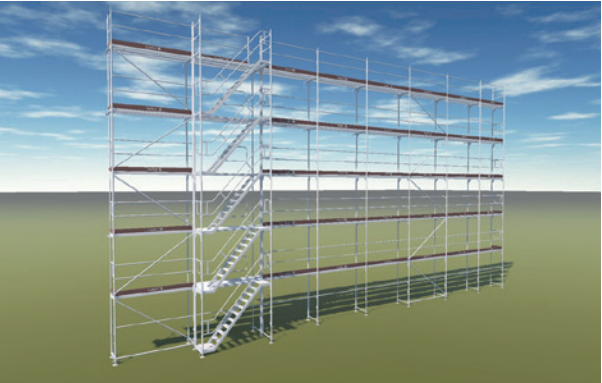
3D visualisation in LayPLAN CLASSIC.
