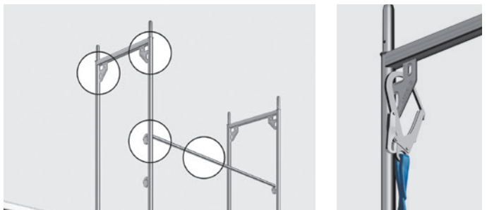
Verified attachment points for personal protective equipment (PPE) against falls.
